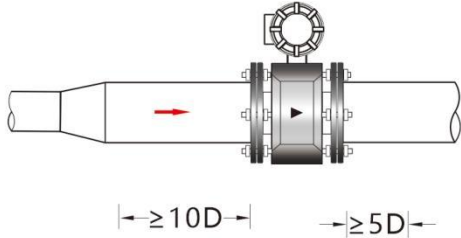
Horizontal straight pipe
